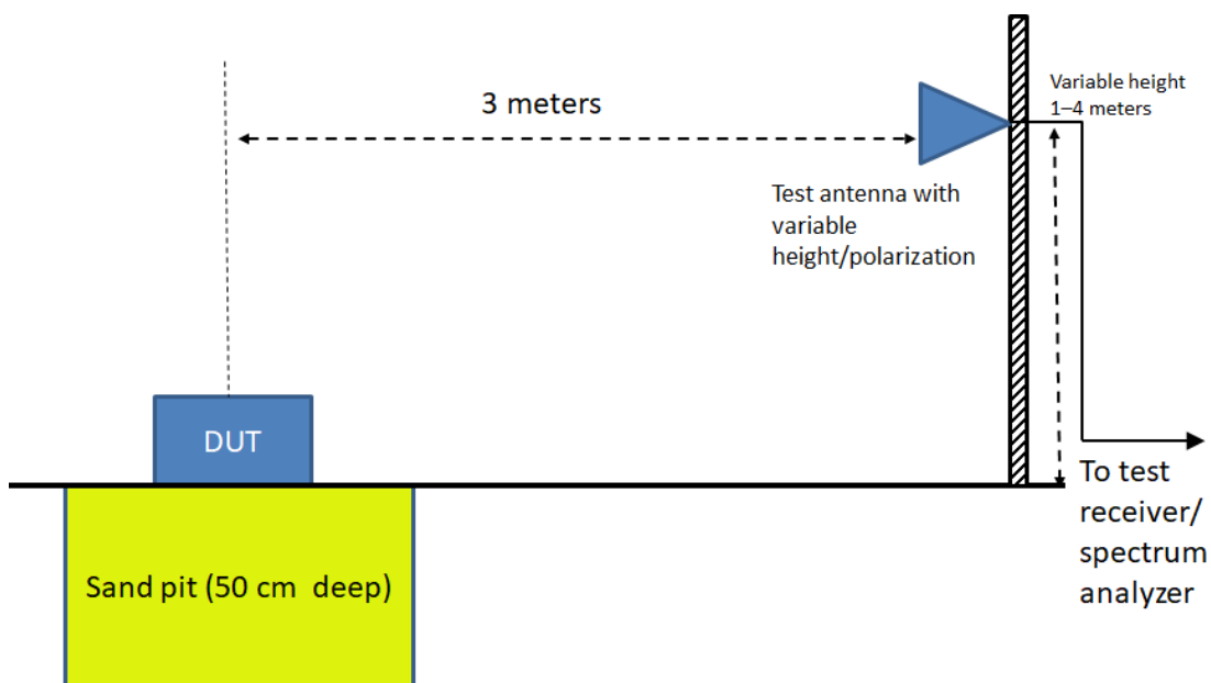
Figure 3: Calibrated setup for other GPR/WPR and measurements below 960 MHz
