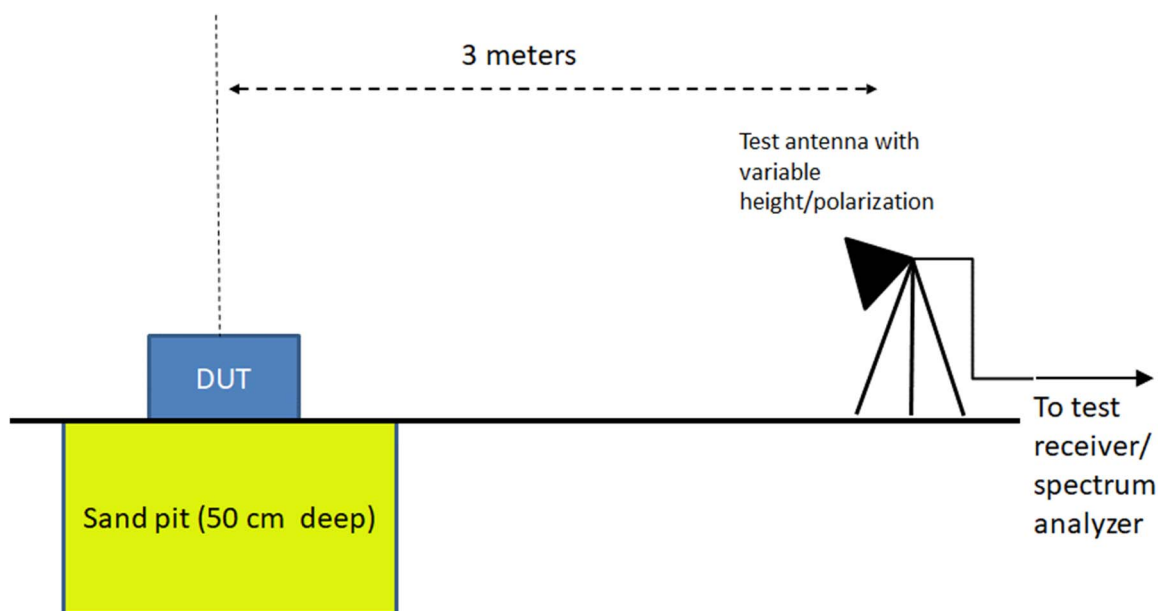
Figure 4: Calibrated setup for other GPR/WPR and measurements above 960 MHz
